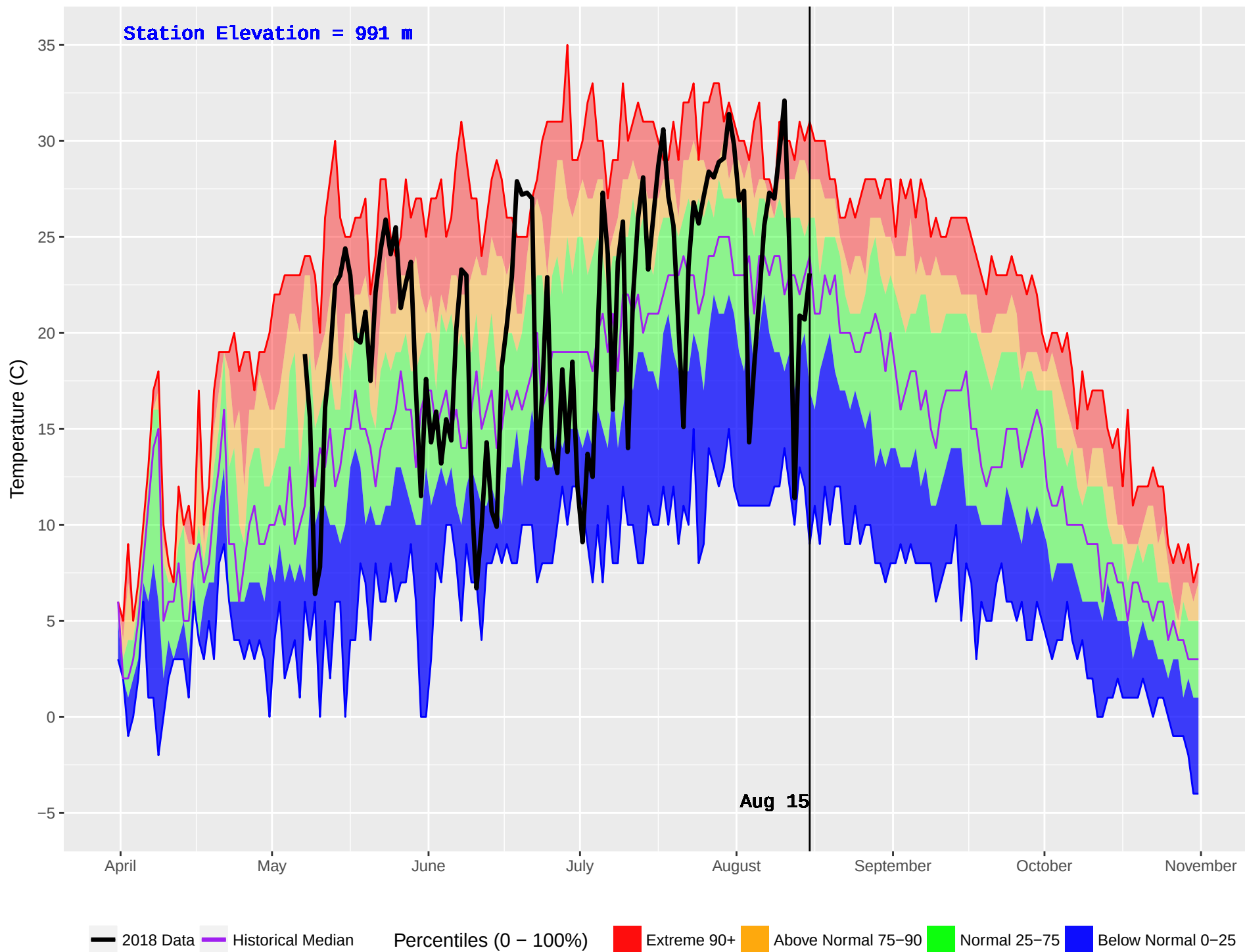
TROUT LAKE (387) : Historical (1987–2016) and Current (2018) Daily Temperature
