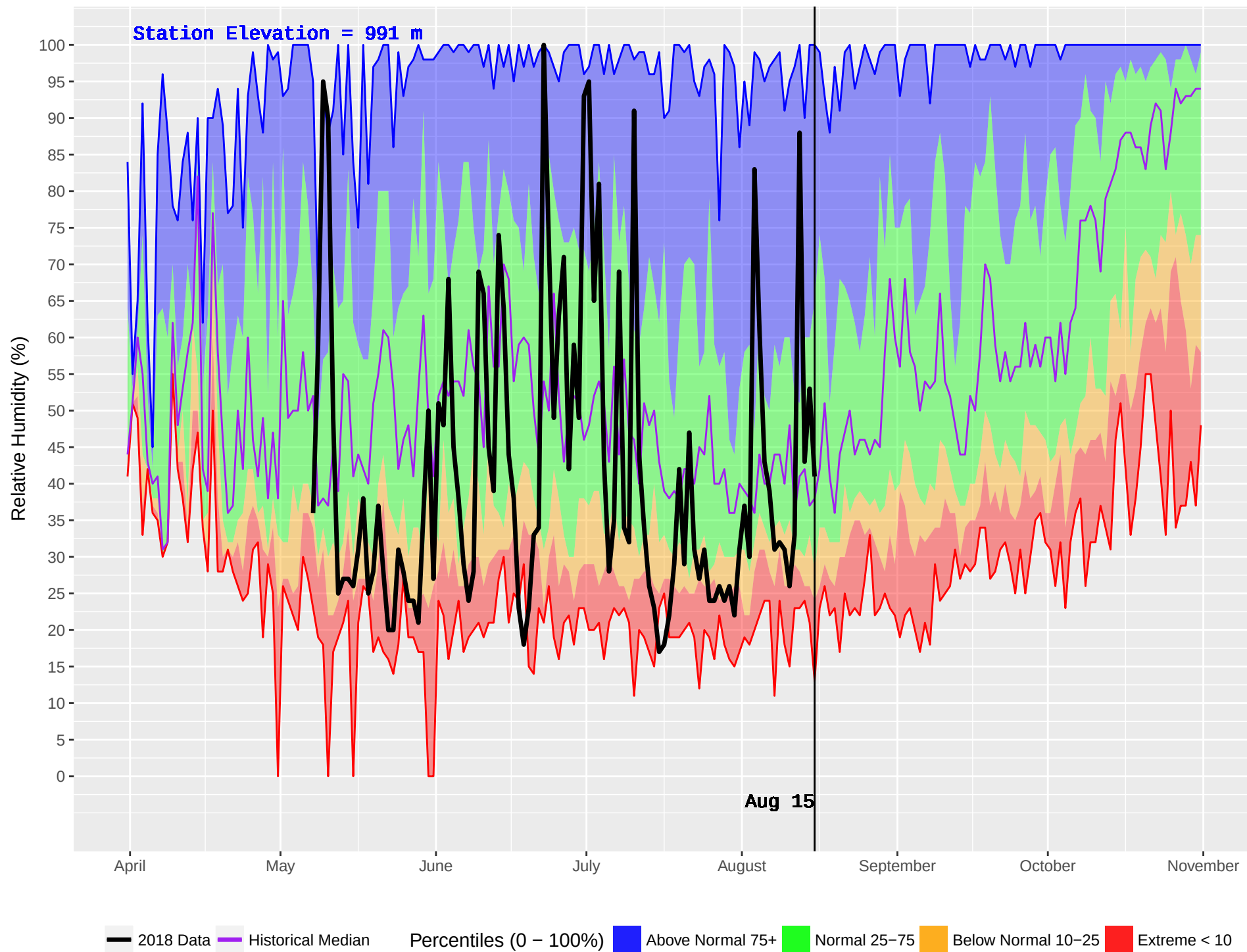
TROUT LAKE (387) : Historical (1987–2016) and Current (2018) Daily Relative Humidity
